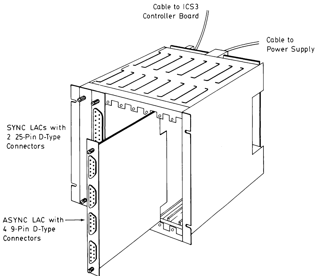
8-LAC ICS3 Card Cage Figure 5-4
