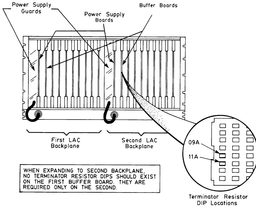
ICS2 Card Cage — Front View Showing Buffer Boards Figure 5-3
