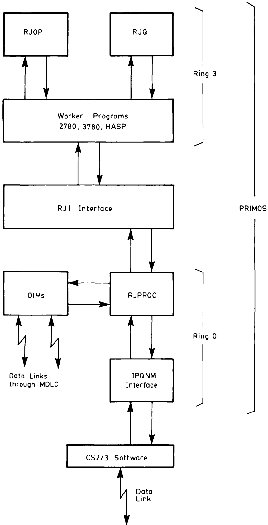
Prime RJE Software Figure 3-2
