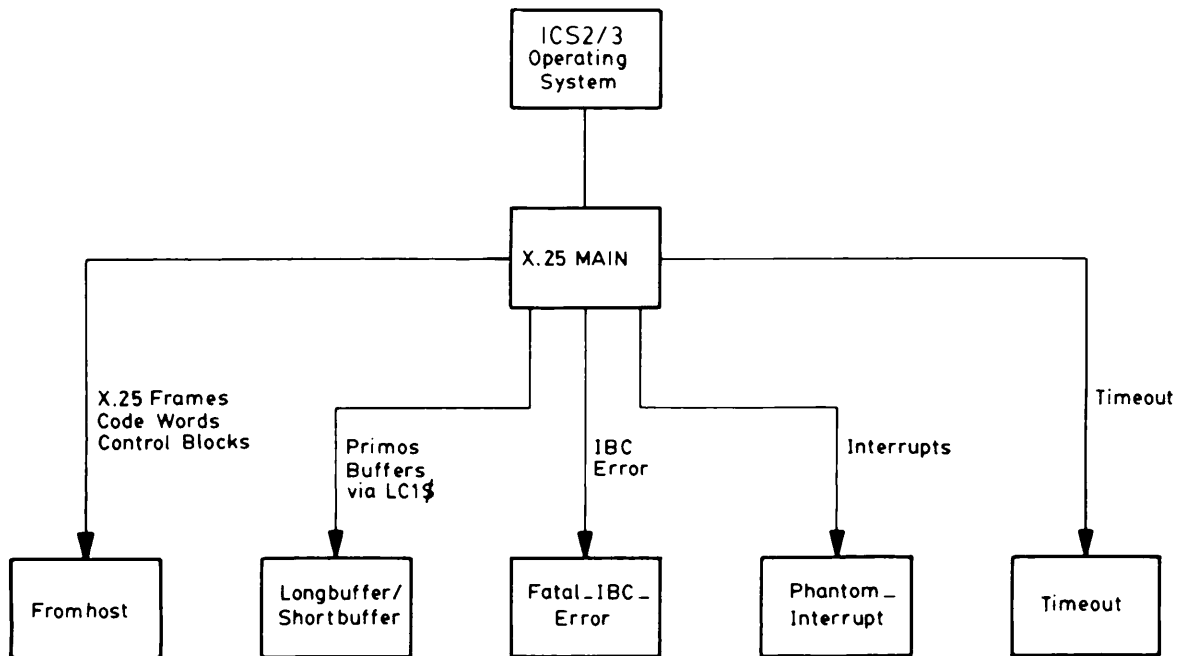
Overview of the ICS2/3 X.25 Software Figure 2-5
