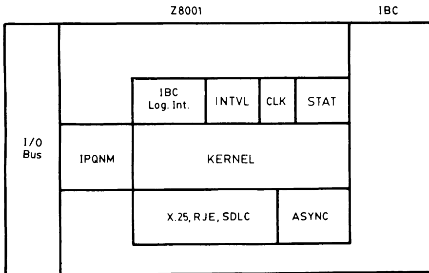
ICS2/3 OS Functional Interconnection Figure 2-3
