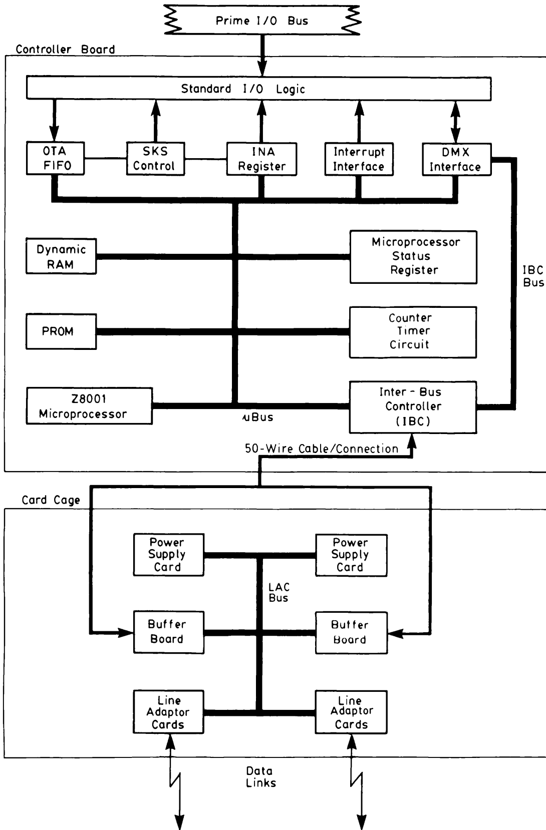
ICS2/3 Hardware Architecture Figure 4-1
