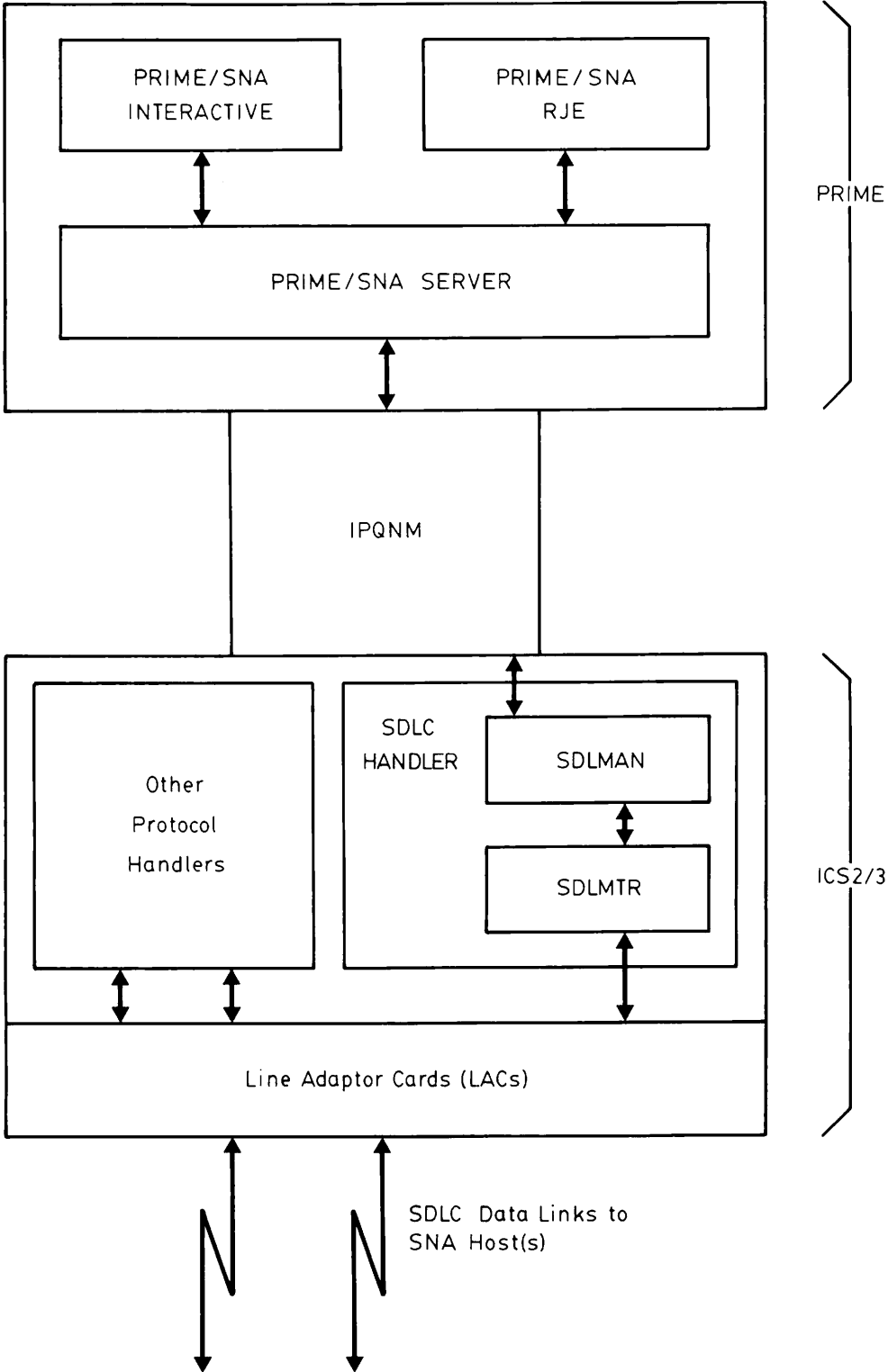
PRIMOS — ICS2/3 Software Connection Figure 2-8
